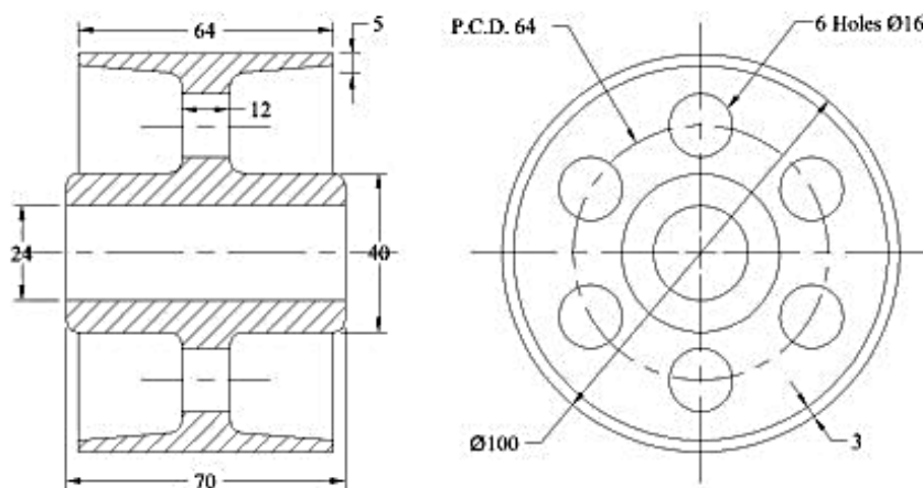
PULLEY (C.I.)
