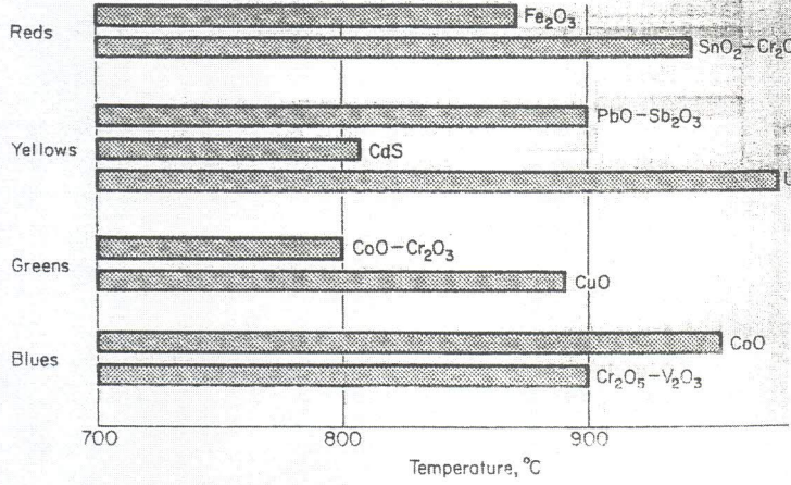
Fig. 14.11 Stability range for overglaze colors.
